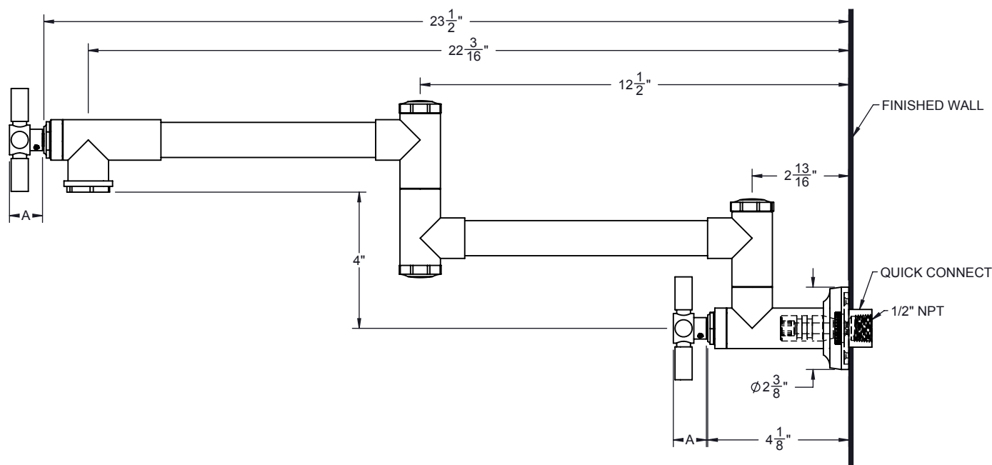
CF-K30-200-SX SHOWN
